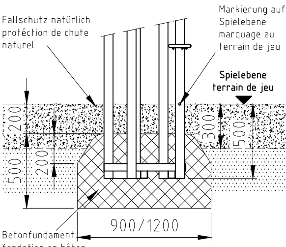
Fundament F50
