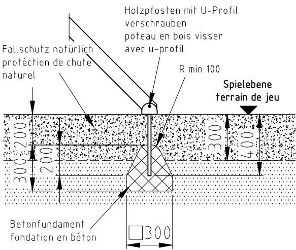
Fundament F05
