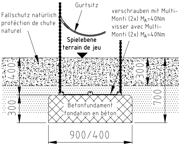
Fundament F50
