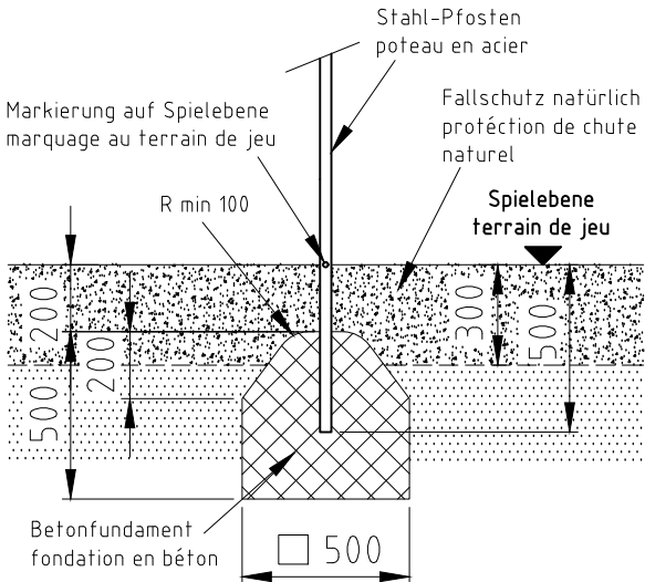
Fundament F05
