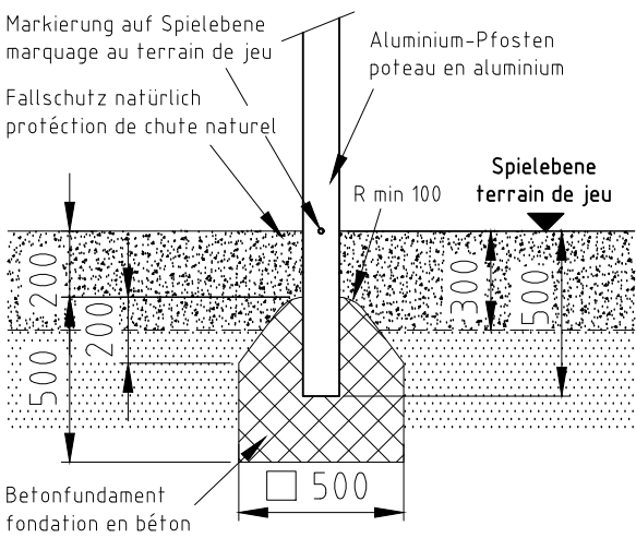
Fundament F03
