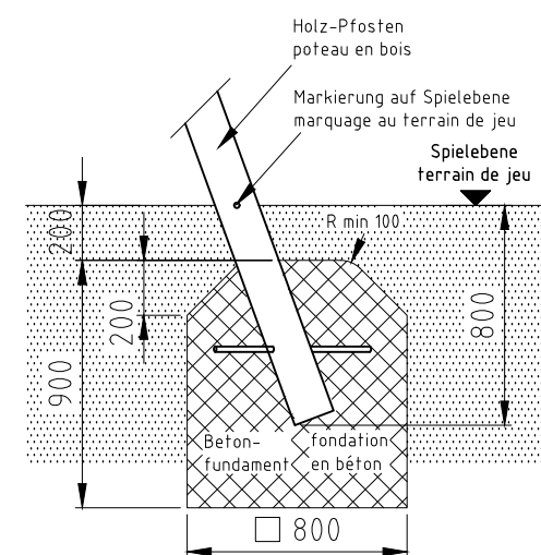
Fundament F91.1
