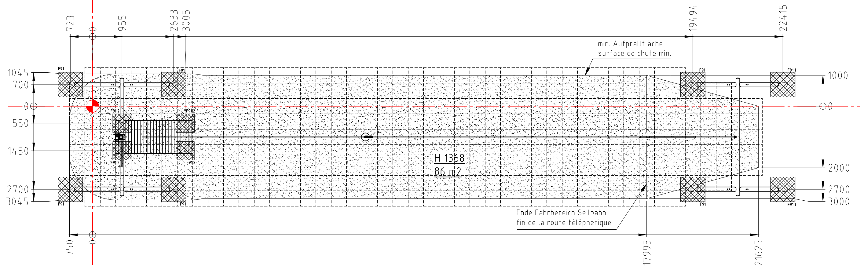
Fundament F91.1
