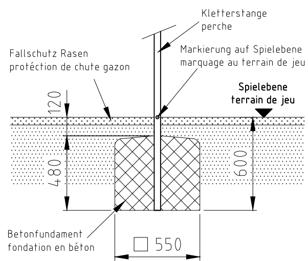
Fundament F05-R
