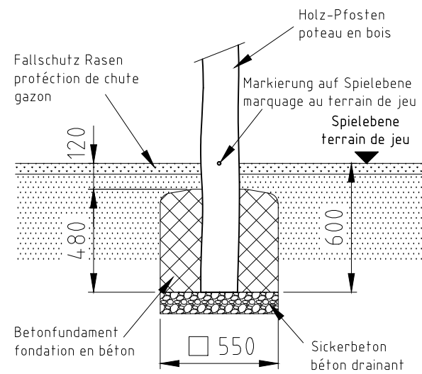
Fundament F01-R
