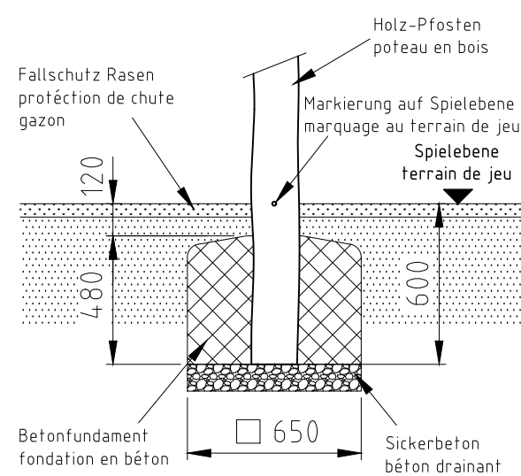
Fundament F02-R
