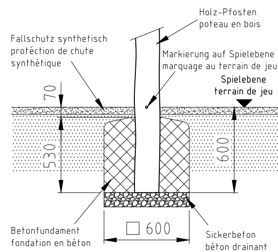
Fundament F02
