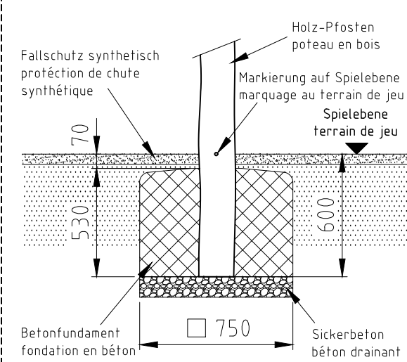
Fundament F03
