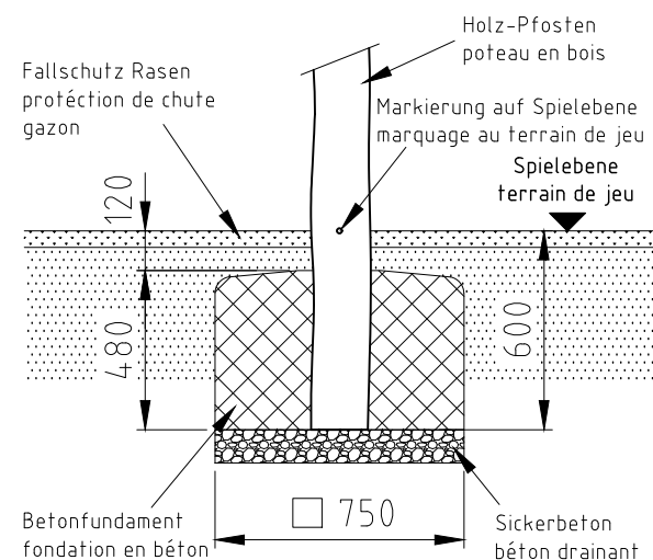
Fundament F03-R
