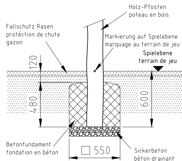
Fundament F01-R
