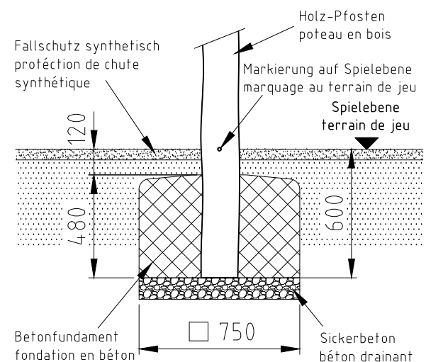
Fundament F03
