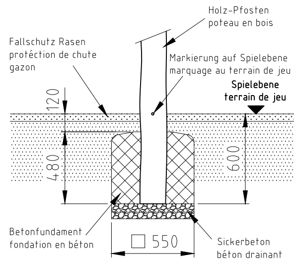
Fundament F01-R
