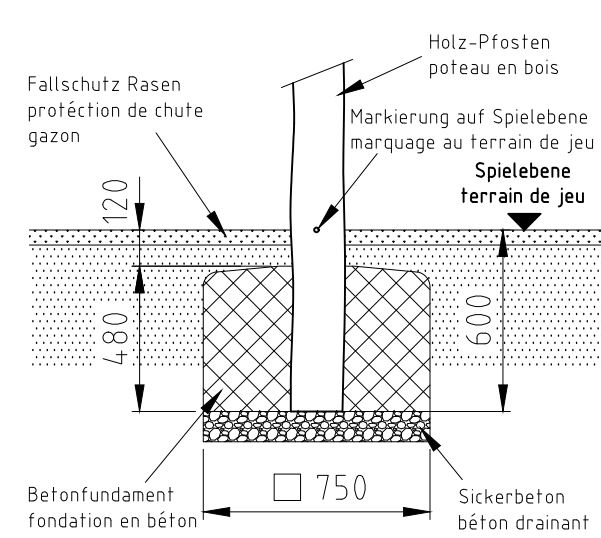
Fundament F03-R
