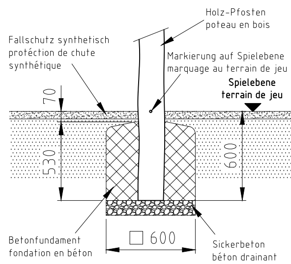
Fundament F02
