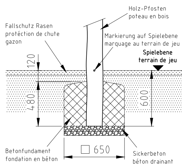
Fundament F02-R
