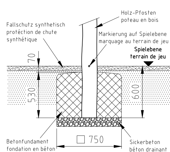
Fundament F03
