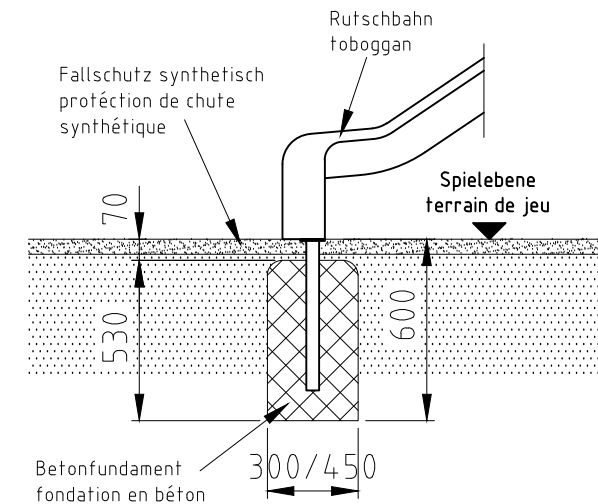
Fundament F09
