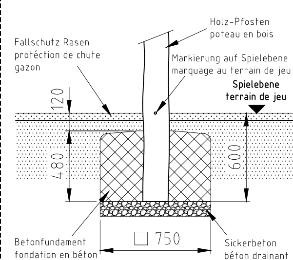
Fundament F03-R
