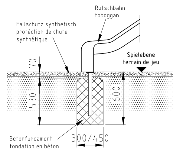
Fundament F09
