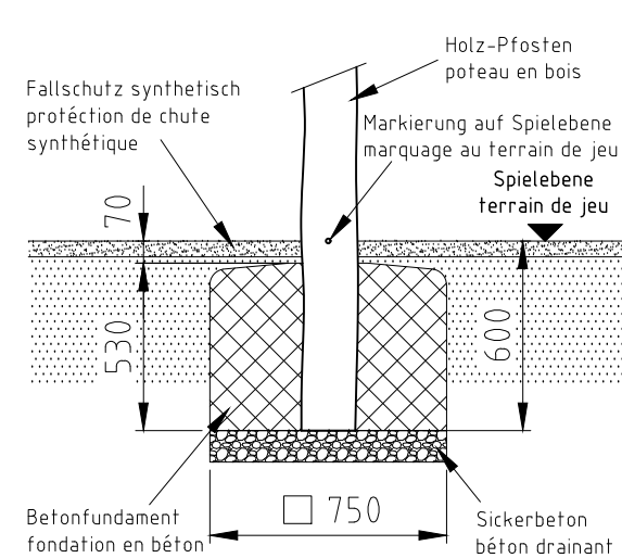
Fundament F03
