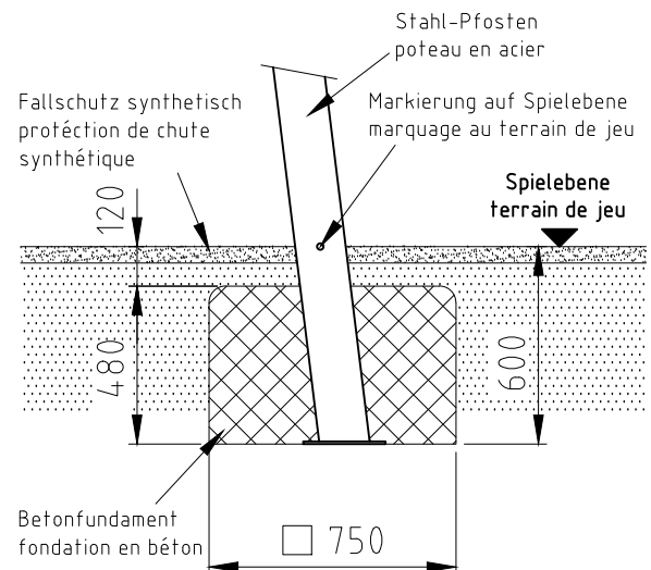
Fundament F03
