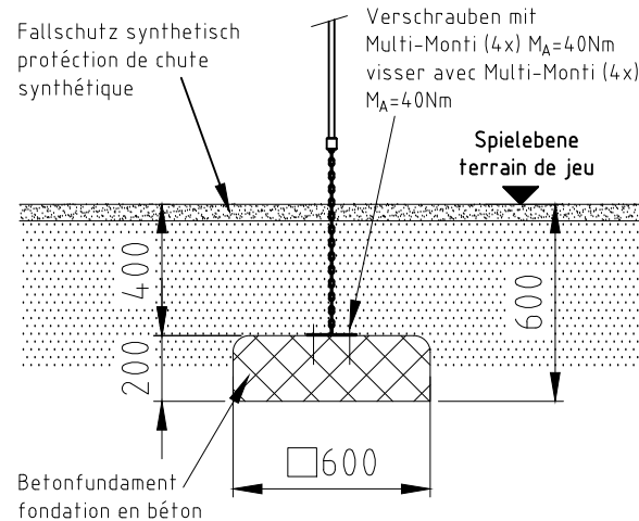
Fundament F09
