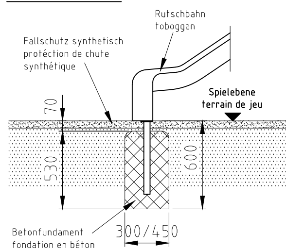
Fundament F09
