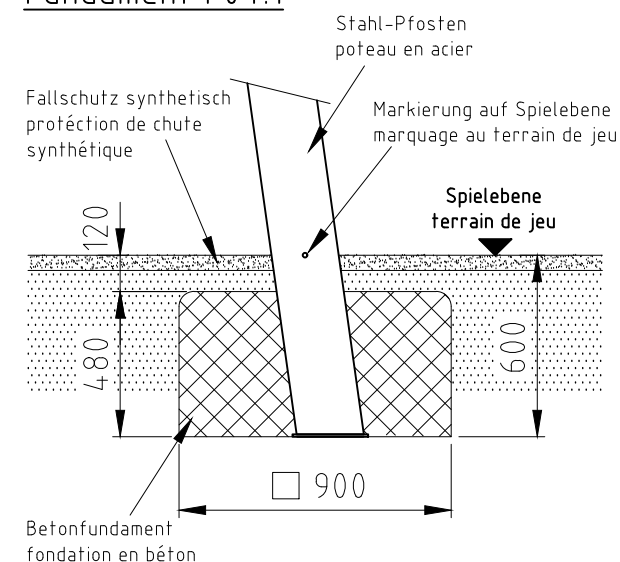
Fundament F04.1
