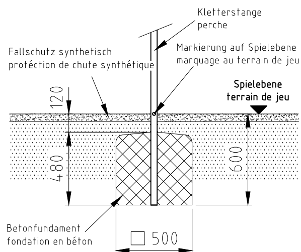
Fundament F05
