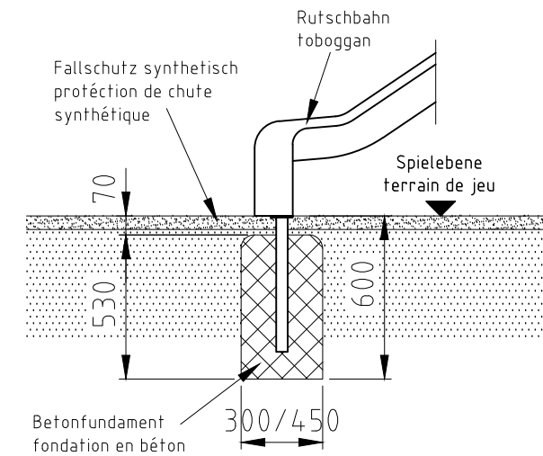
Fundament F09
