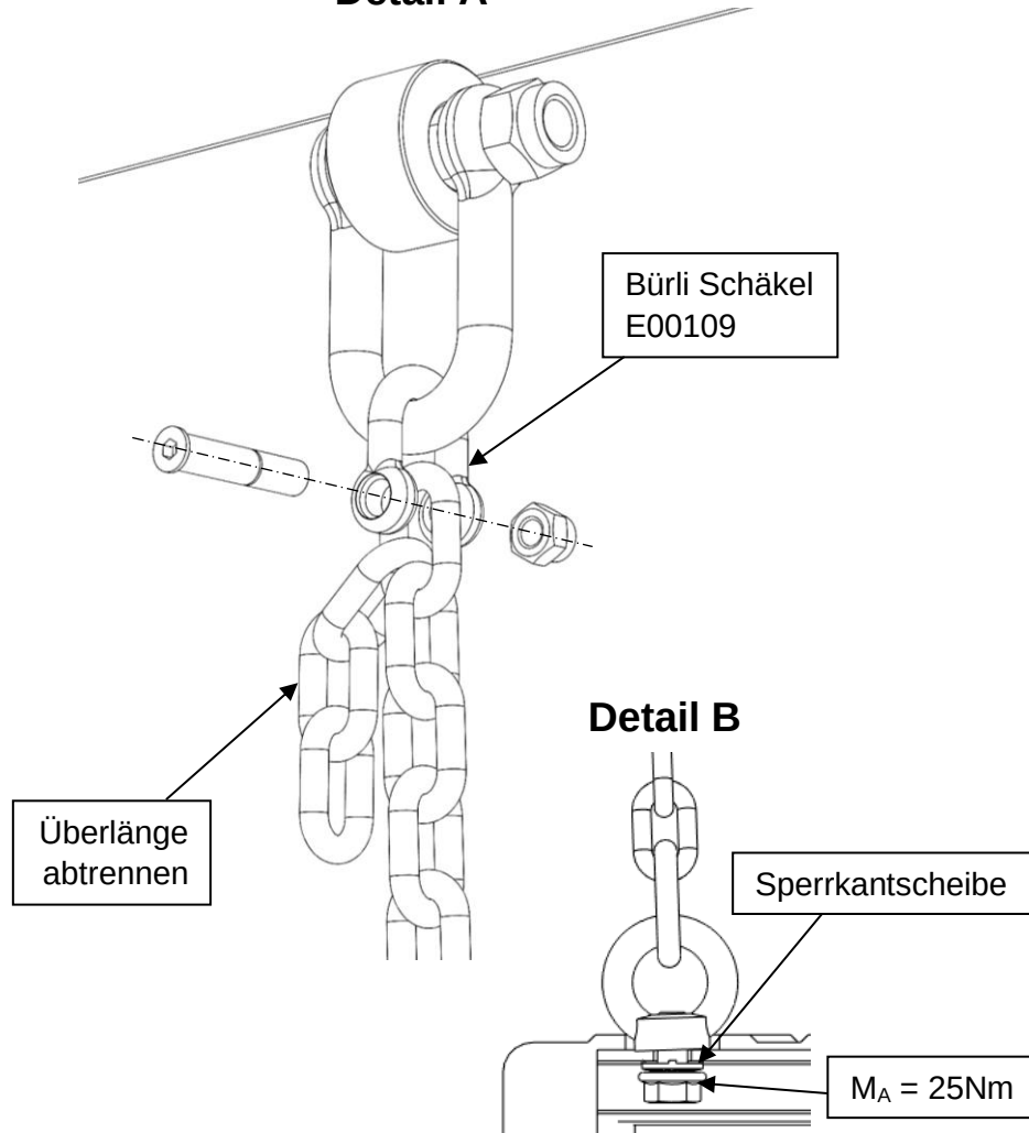
Detail A
