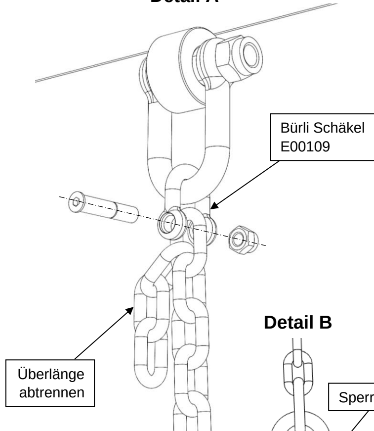
Detail A
